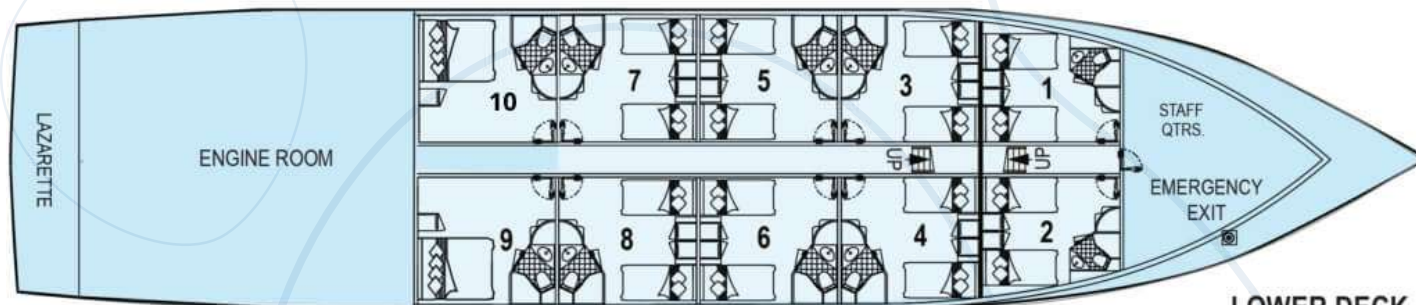
LOWER DECK
