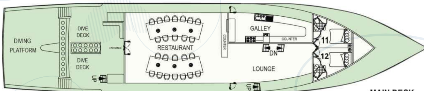
MAIN DECK
